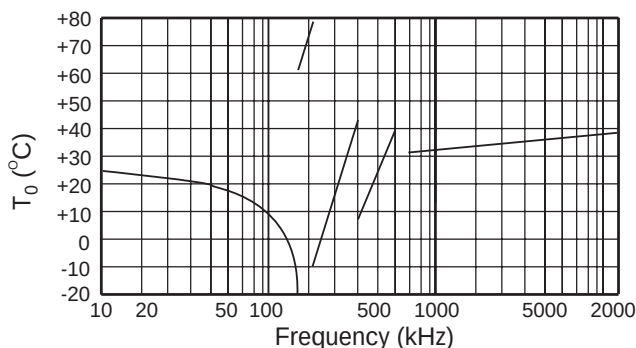
FIGURE 2. TYPICAL TURNING POINT TEMPERATURE (T O )
