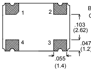
Figure 1 - Package Configuration & Pin Connections
